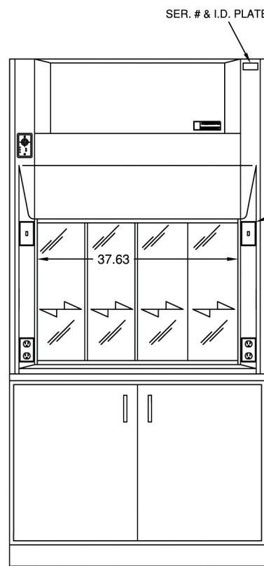
MODEL 12240 (WITH OPTIONAL BASE CABINET AND WORKSURFACE)
