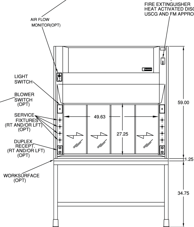
MODEL 12250 (WITH OPTIONAL TABLE AND WORKSURFACE)
