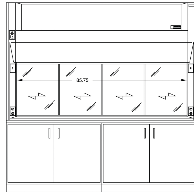
MODEL 12280 (WITH OPTIONAL BASE CABINETS AND WORKSURFACE)
